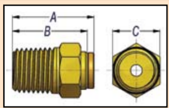
STYLE DQ68DOT MALE CONNECTOR Imperial Tube to NPTF Male Pipe Thread
