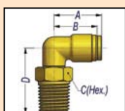
STYLE DQ69DOTS SWIVEL MALE ELBOW Imperial Tube to NPTF Male Pipe Thread
