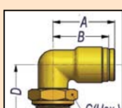
STYLE DQ69DOTS SWIVEL MALE ELBOW Imperial Tube to Metric Thread
